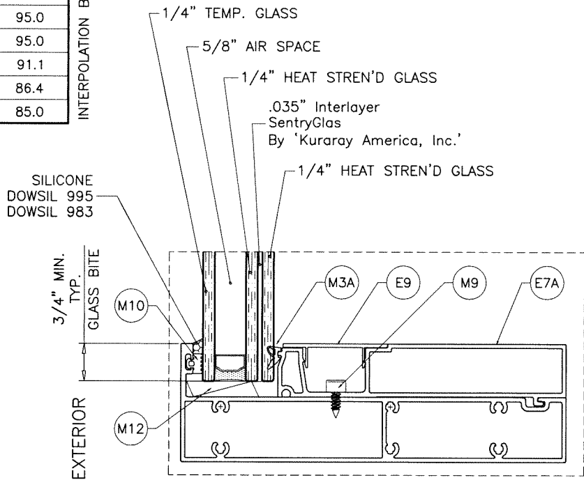
GLASS TYPE 'C' 1-7/16" OVERALL INSUL. LAM. GLASS
