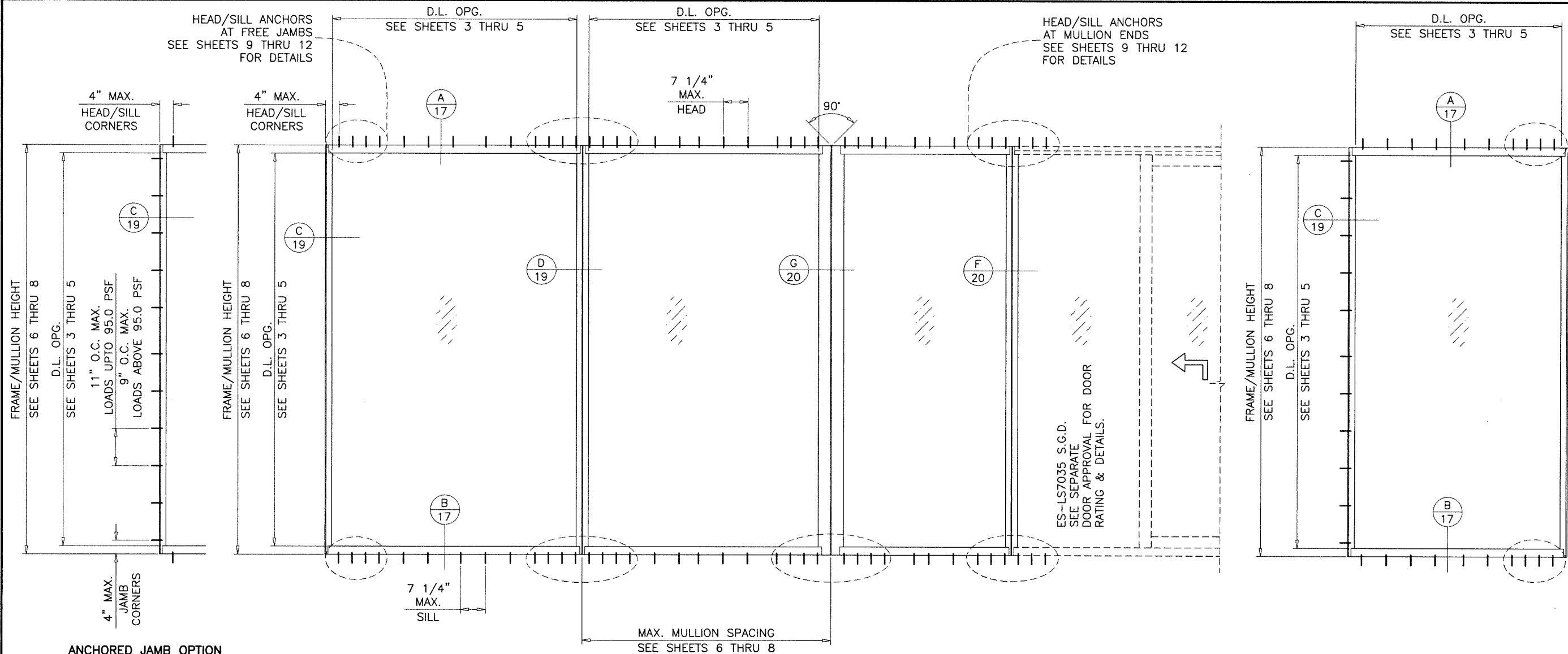
ANCHORED JAMB OPTION
