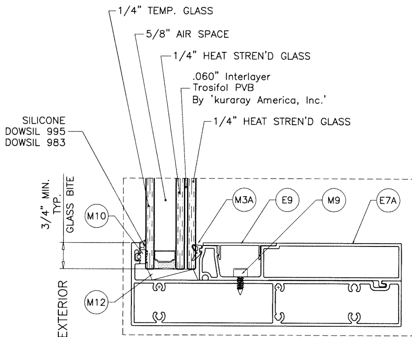
GLASS TYPE 'D' 1-7/16" OVERALL INSUL. LAM. GLASS
